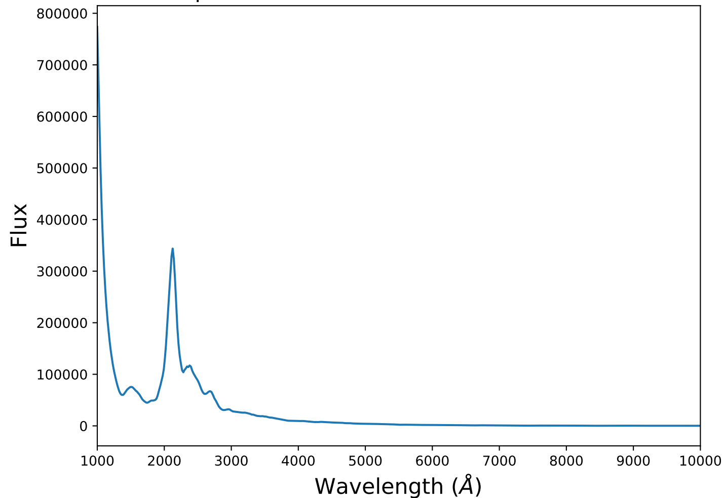
Spectrum 3 for transient SNIa at z=0.36
